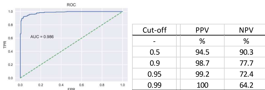
Figure 4: Receiver Operator Curve (ROC) and effect of cut-off point on PPV and NPV
