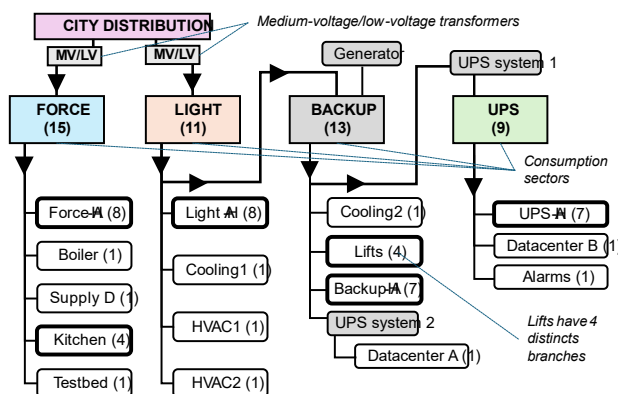
Figure 1. Campus electric power distribution. Numbers in parentheses designate the number of electrical branches. Bold boxes indicate the 38 existing Measurement Points.
