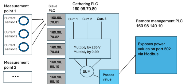
Figure 3. Existing power measurement infrastructure.
