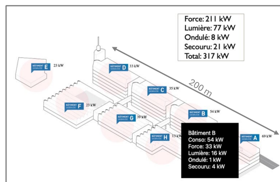
Figure 6. Widget showing the complete actual electric consumption across the campus. The top box shows the school’s total consumption, per sector and aggregated.
