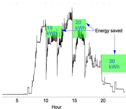
Figure 5. Building D lighting consumption on 23.04.2023. Green rectangles saved energy.
