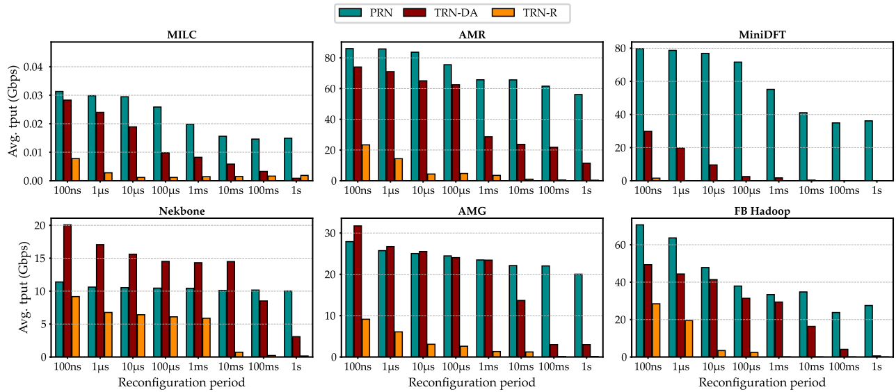
Fig. 12. Cost-equivalent evaluation of a PRN and a TRN. Average flow throughput of HPC and DC workloads as a result of various reconfiguration periods.
